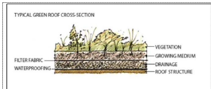
Figure 1. Typical Rooftop garden in cross section
