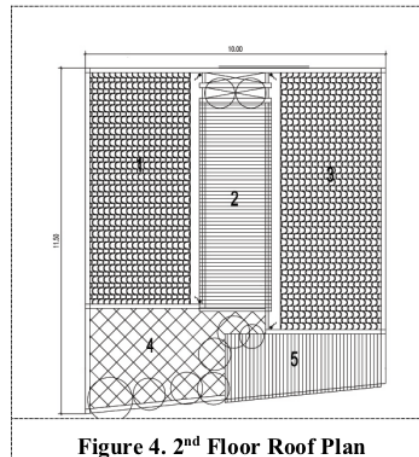
Figure 4. 2 nd Floor Roof Plan
