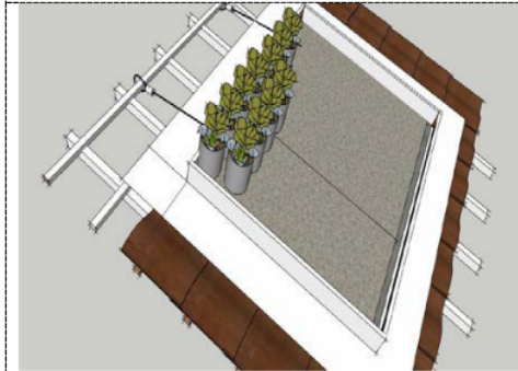
Figure 2. Design of Green Roof Media
