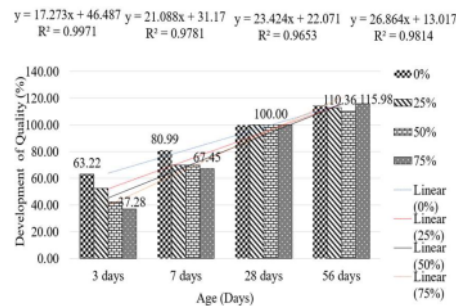
Fig. 15 Development of Quality Concrete (K400)
