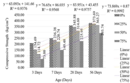
Fig.12 Quality of Compressive Strength (K300)
