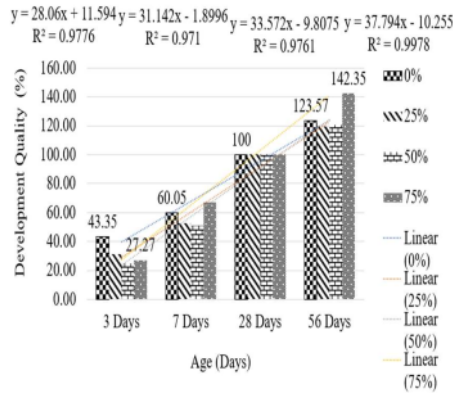
Fig. 11 Development of Quality Concrete (K-200)
