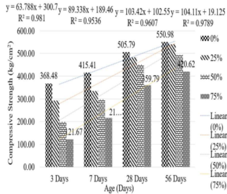
Fig. 17 Development of Quality Concrete (K500)
