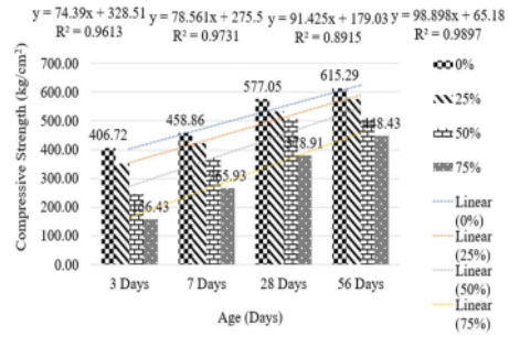
Fig. 18 Quality of Compressive Strength (K600)
