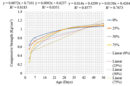
Fig. 7 Development of Mortar Strength
