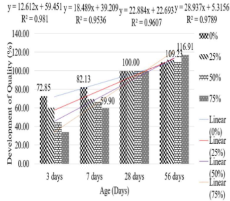
Fig. 16 Quality of Compressive Strength (K500)
