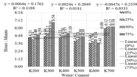
Fig. 8: Initial setting time of concrete
