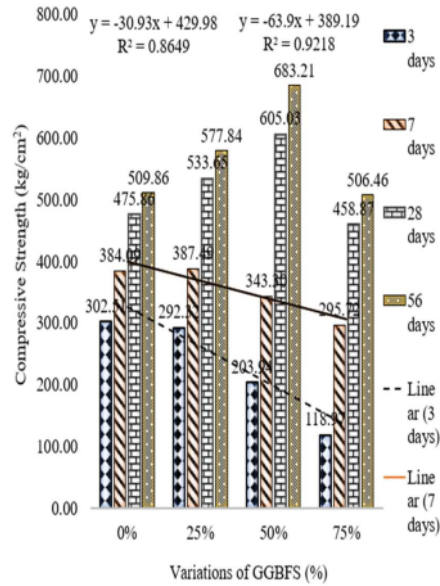
Fig. 6 Mortar Strength Mortar Comparison Number
