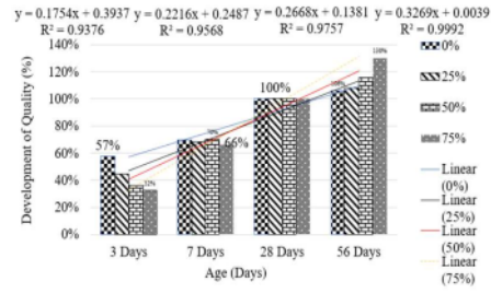
Fig.13 Development of Quality Concrete (K-300)
