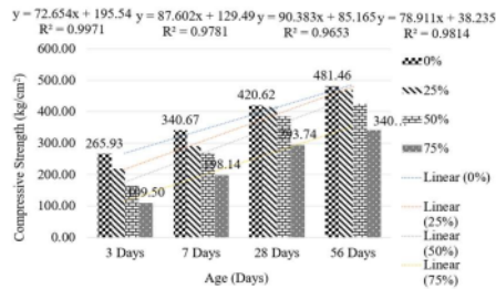
Fig. 14 Quality of Compressive Strength (K400)
