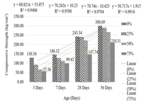
Fig.10 Quality of Compressive Strength (K200)
