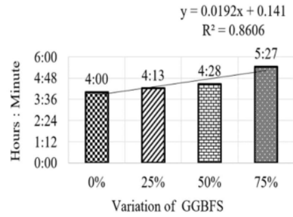
Fig. 5 Initial setting Time of Mortar
