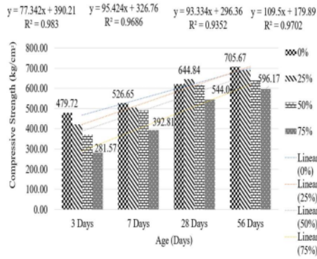
Fig.20 Quality of Compressive Strength (K700)
