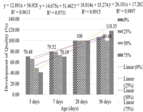
Fig. 19 Development of Quality Concrete (K600)
