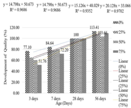
Fig. 21 Development of Compressive Strength (K700)
